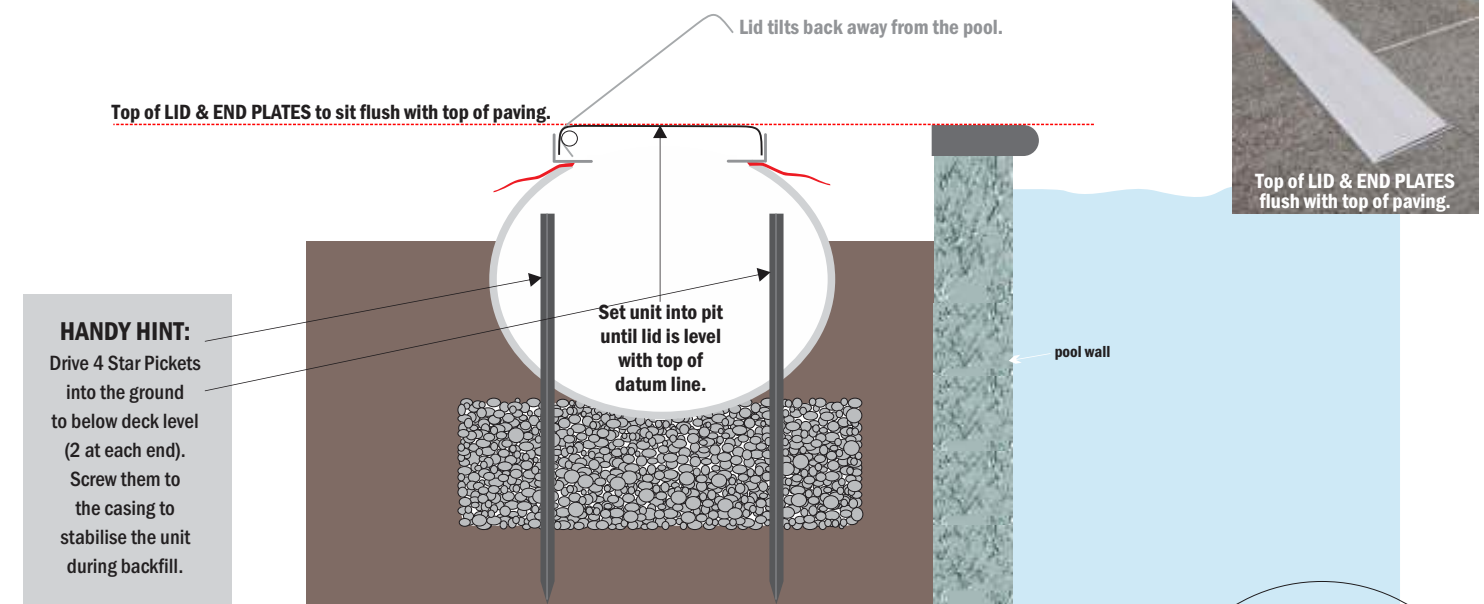
Step 4B. PLACING THE UNIT & BACKFILLING
