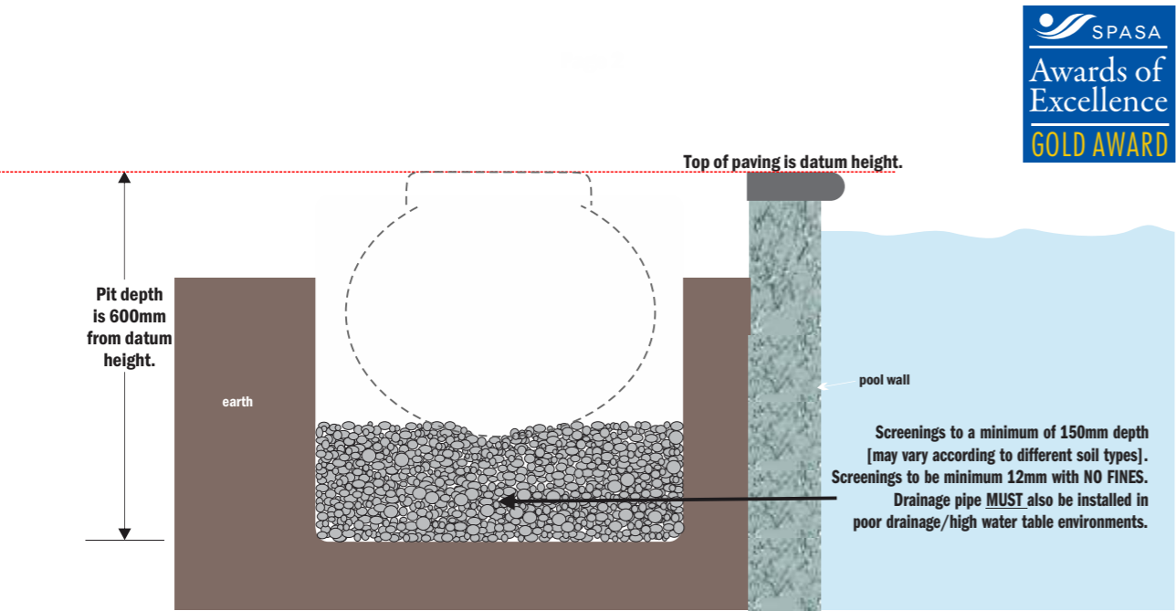
Step 3B. GOOD DRAINAGE IS ESSENTIAL
